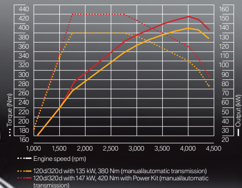
Performance data for the BMW 120d/320d with BMW M Performance Power Kit Full load 120d/320d
